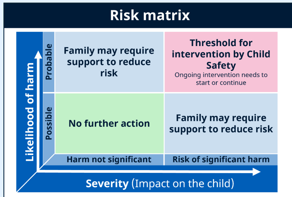
Figure 2: Risk matrix
